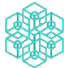
Blockchain
